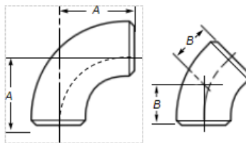
DIMENSIONS OF LONG RADIUS ELBOW
